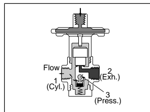
Figure 12D: Normally Closed, Operator Pressurized
